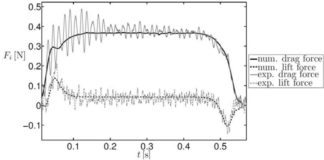
Fig. 2. Raw signal and numerically (transient) obtained characteristic profile at v = 500\text{-mm/s} and \delta z = 3\text{ mm}
