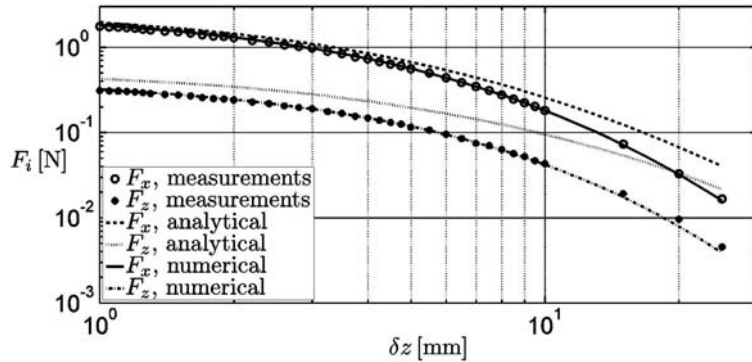
Fig. 6. Comparison between analytically, numerically and experimentally obtained force components with respect to lift-off distance \delta z for a cylindrical permanent magnet \phi 15 \times 25 mm
